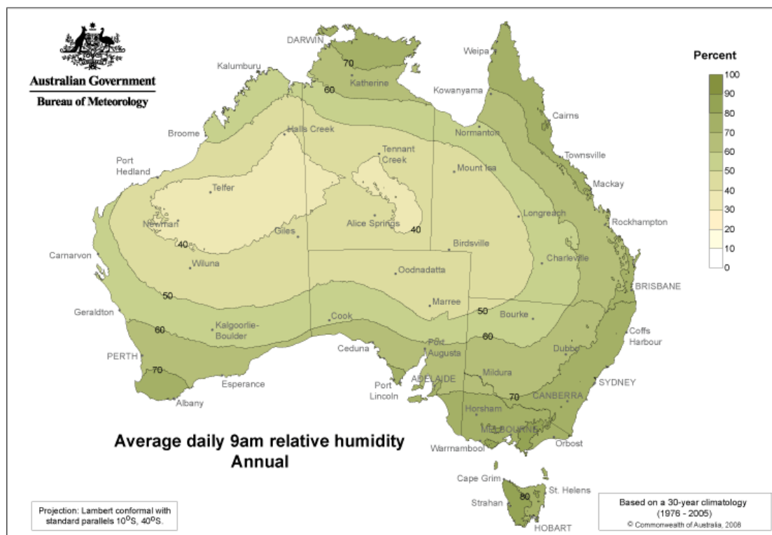
Figure 3 Average relative humidity across Australia
