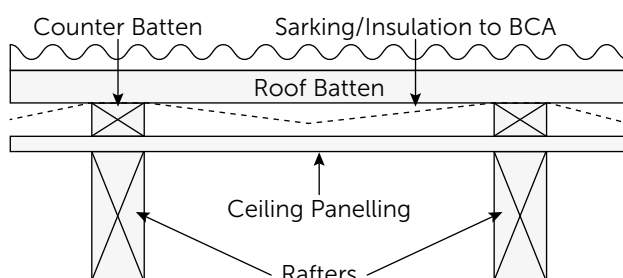
Ceiling Lining fixed on top of rafters
