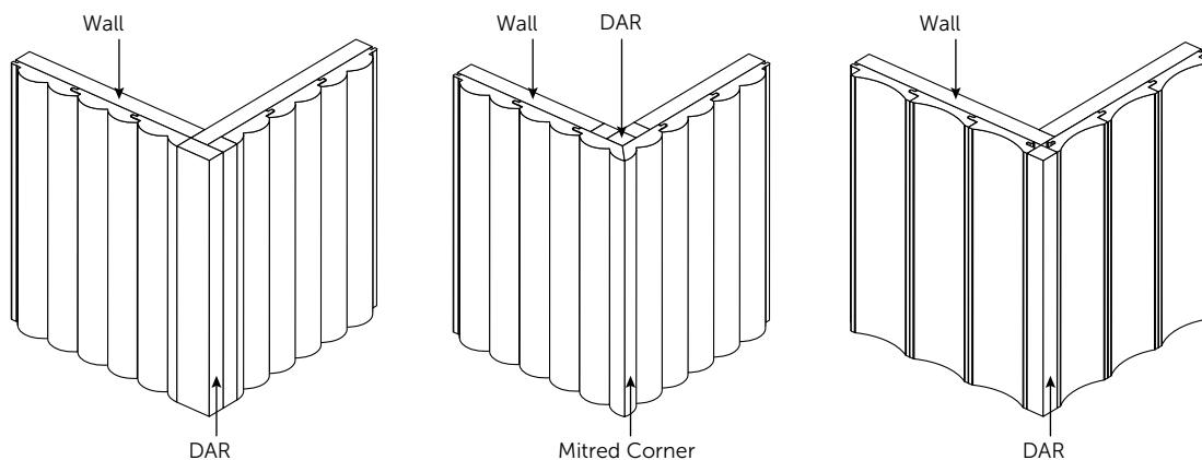
Figure 5 Corner Block details
