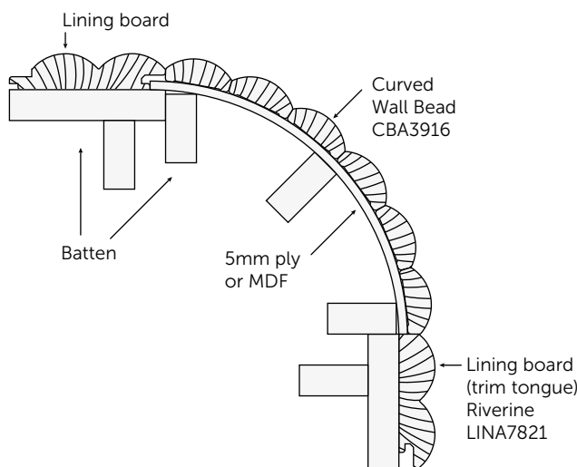
Figure 4 Typical Porta Contours Riverine corner detail schematic
