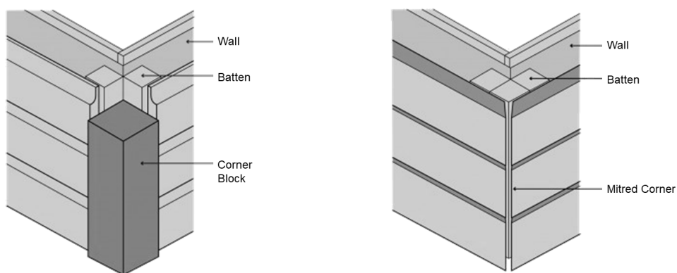
Figure 5 Corner Block details
