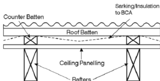
Ceiling Lining fixed on top of rafters
