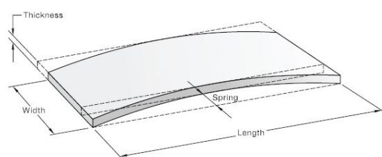
Figure 6 Measurement of Spring
