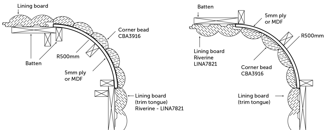
Figure 4 Typical Porta Contours Riverine corner detail schematic
